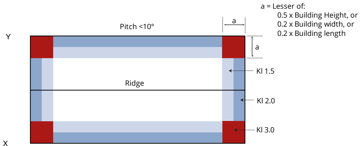
Local Pressure (KI) factors as per AS/NZS 1170:2011
